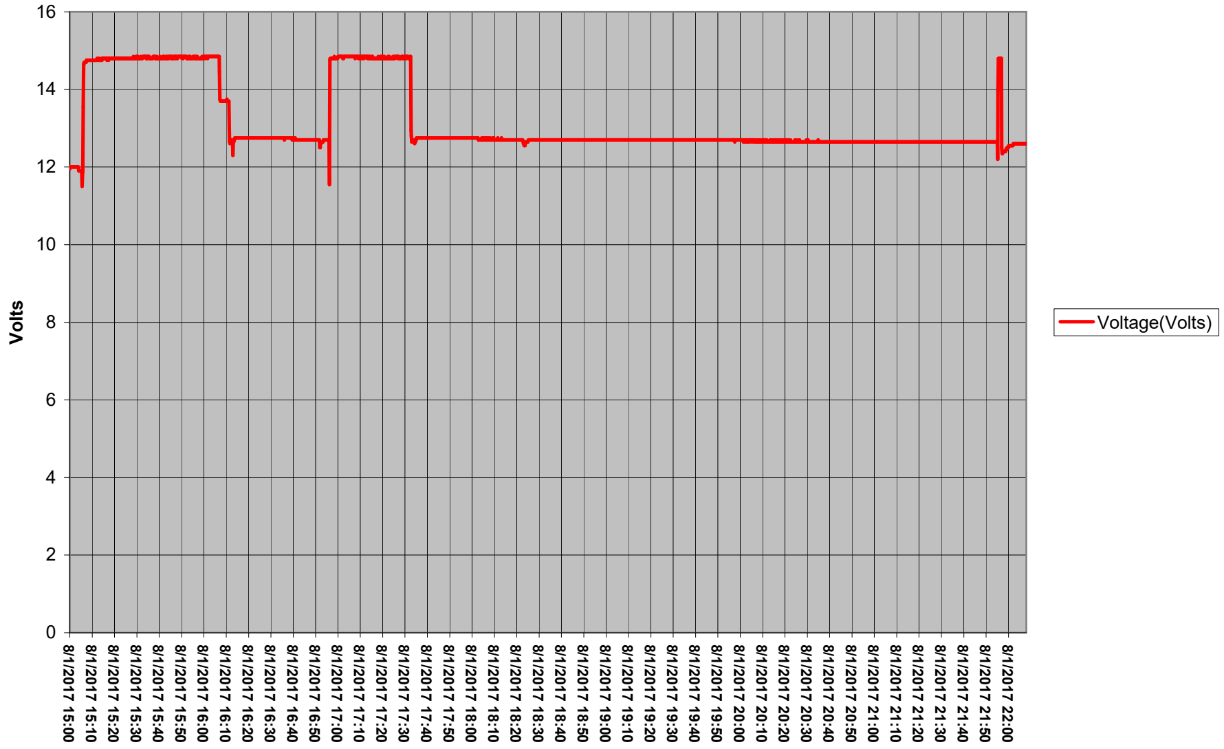
Prius Gen3 battery voltage
