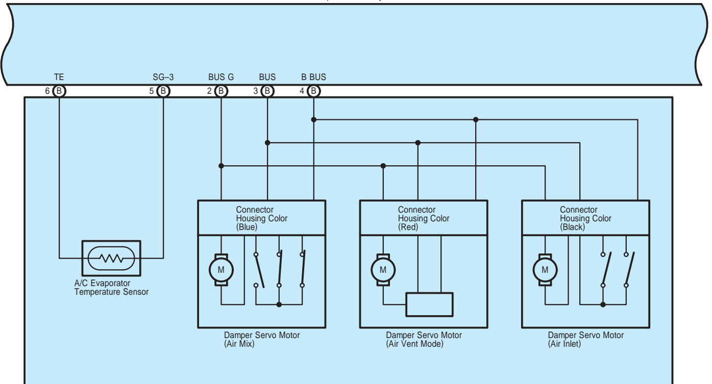
z11(B) A/C Blower Assembly
