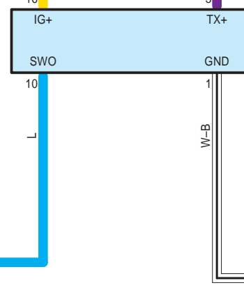
L20 A/C Control Assembly
