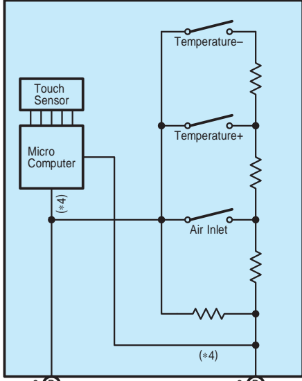
z9(B) Steering Pad Switch Assembly
