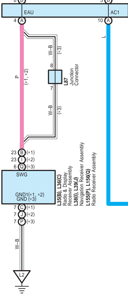
L52(A), z9(B) Spiral with Sensor Cable Sub-Assembly
