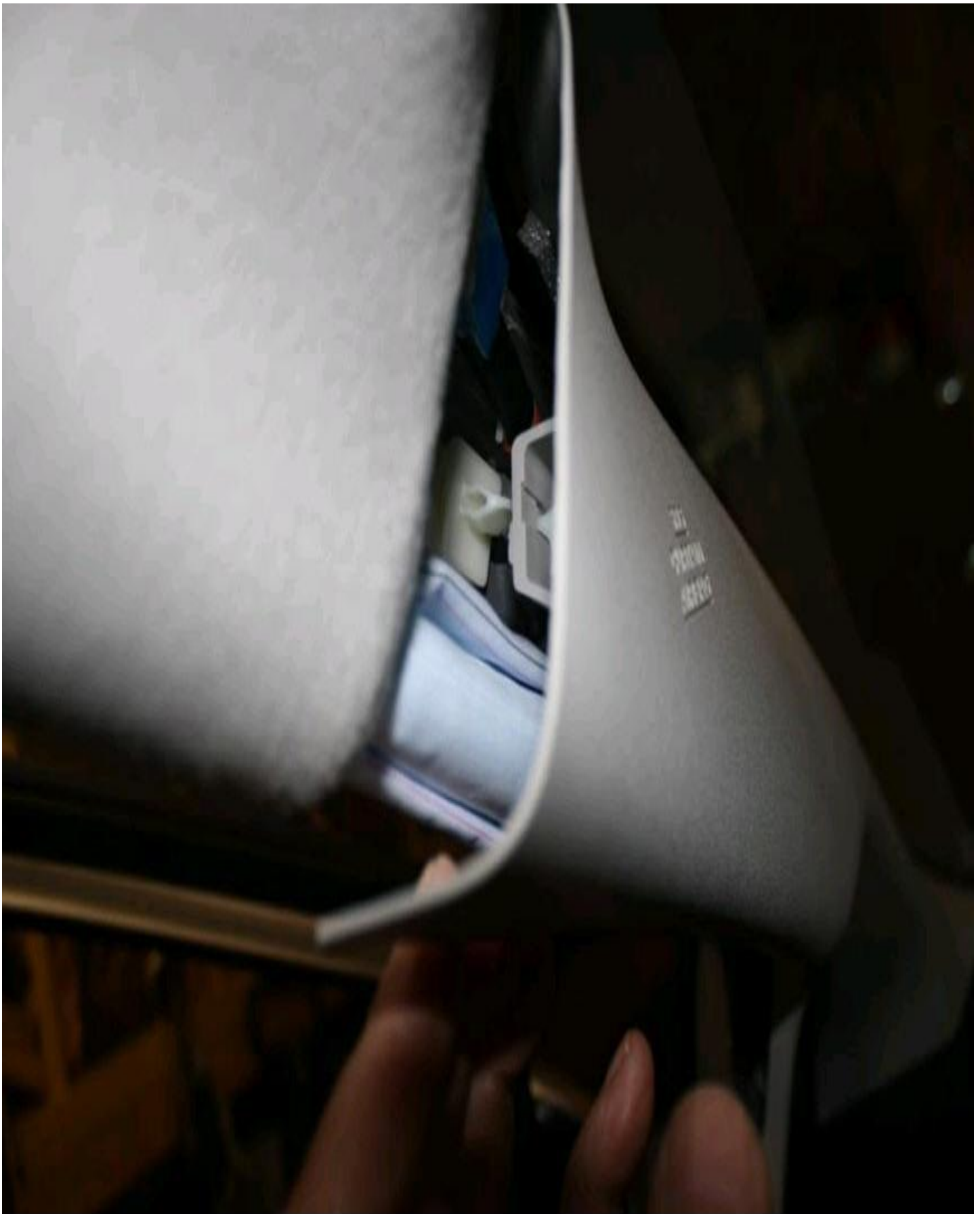
pillar trim at center top but do not remove. Once it is popped it will remain in place with a hook device. This is the retainer to hold the panel if the air is deployed. See next photo.
