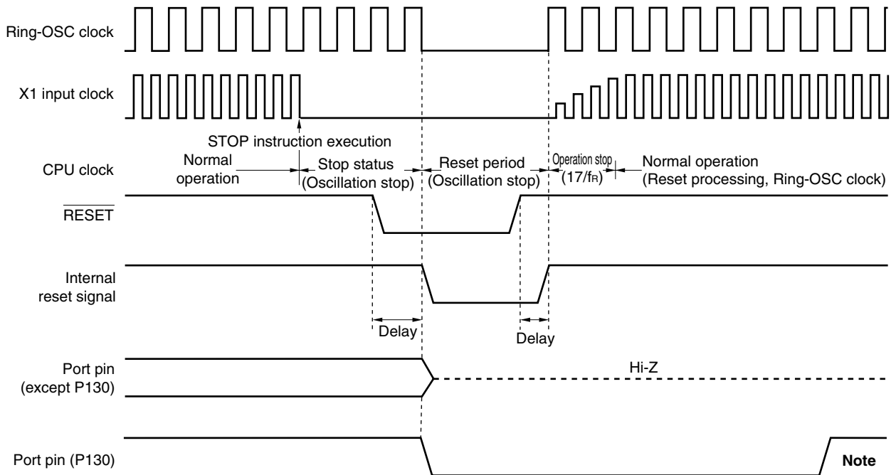
Figure 18-4. Timing of Reset in STOP Mode by RESET Input
