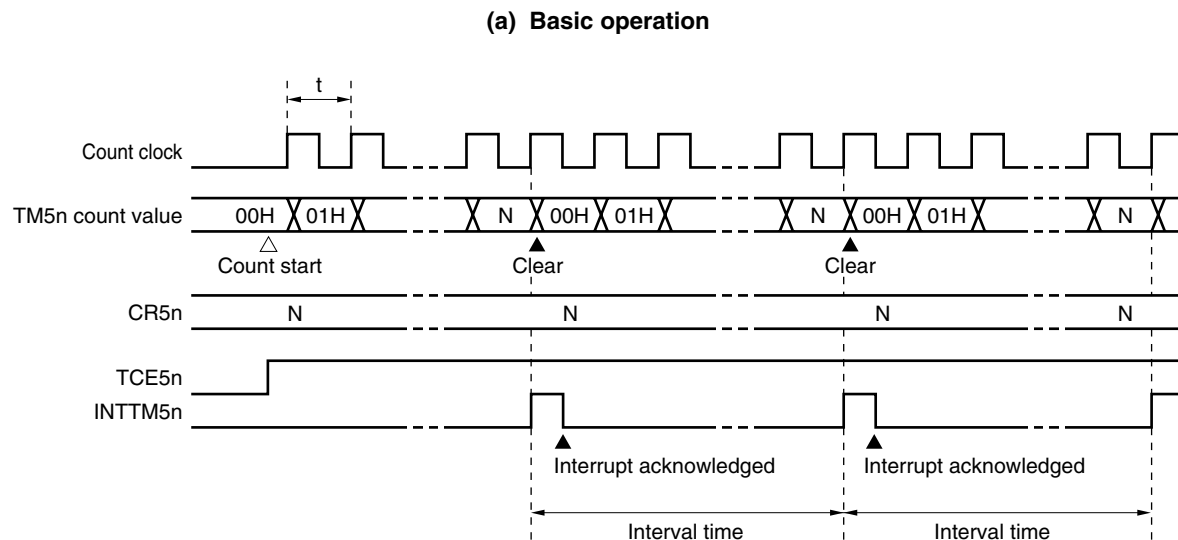
Figure 7-11. Interval Timer Operation Timing (1/2)
