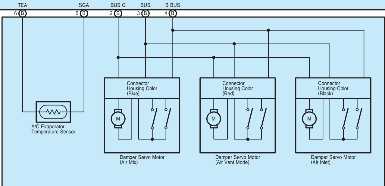
z11(B) A/C Blower Assembly
