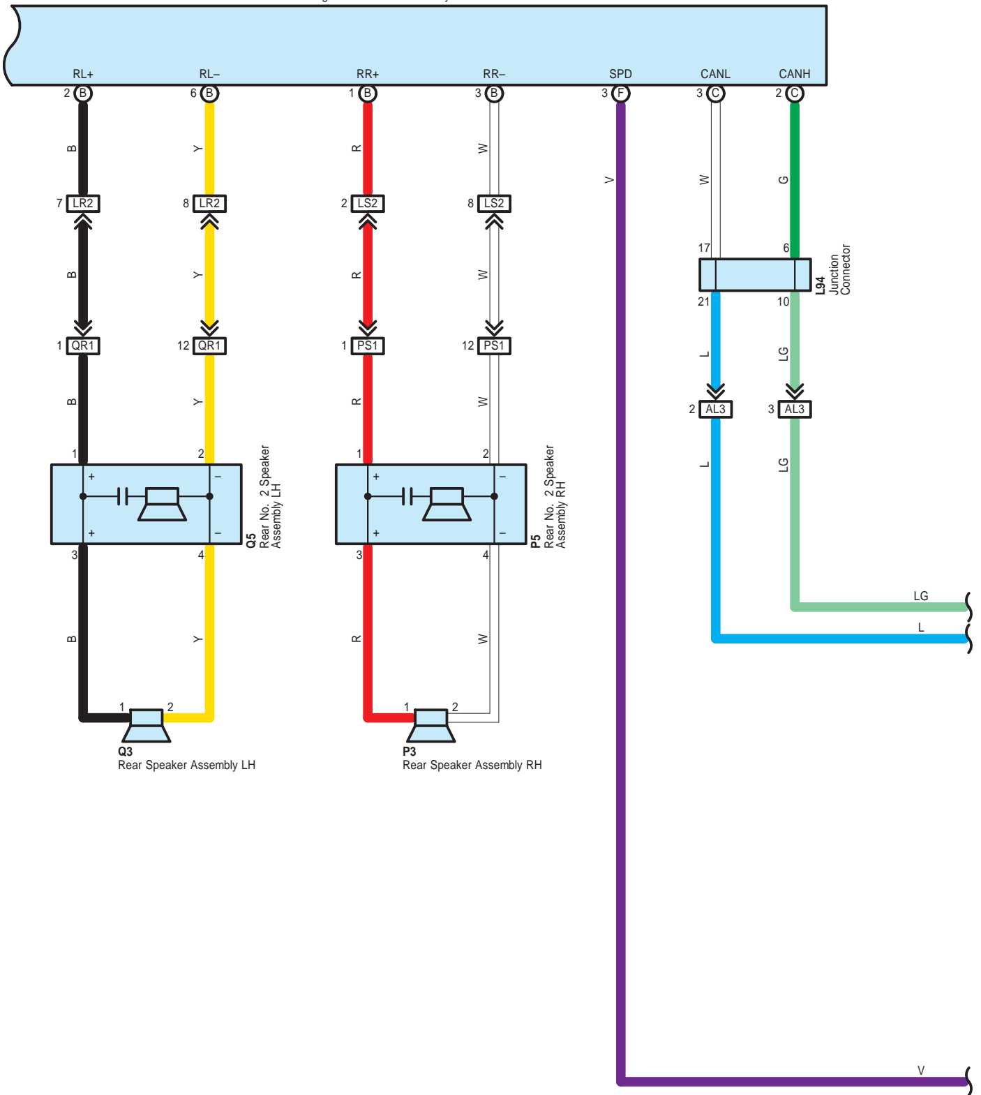
L34(A), L35(B), L37(C), L41(E), L42(F) Navigation Receiver Assembly
