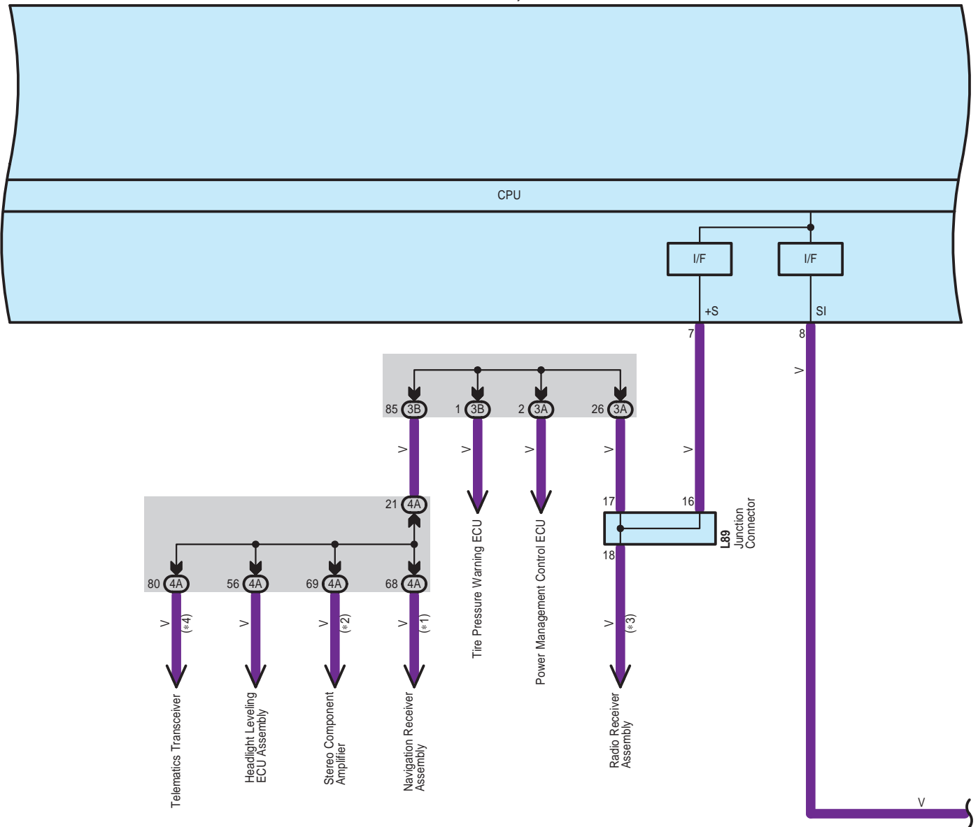
L27 Combination Meter Assembly
