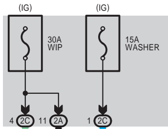
L48(A), L49(B) Windshield Wiper Switch Assembly
