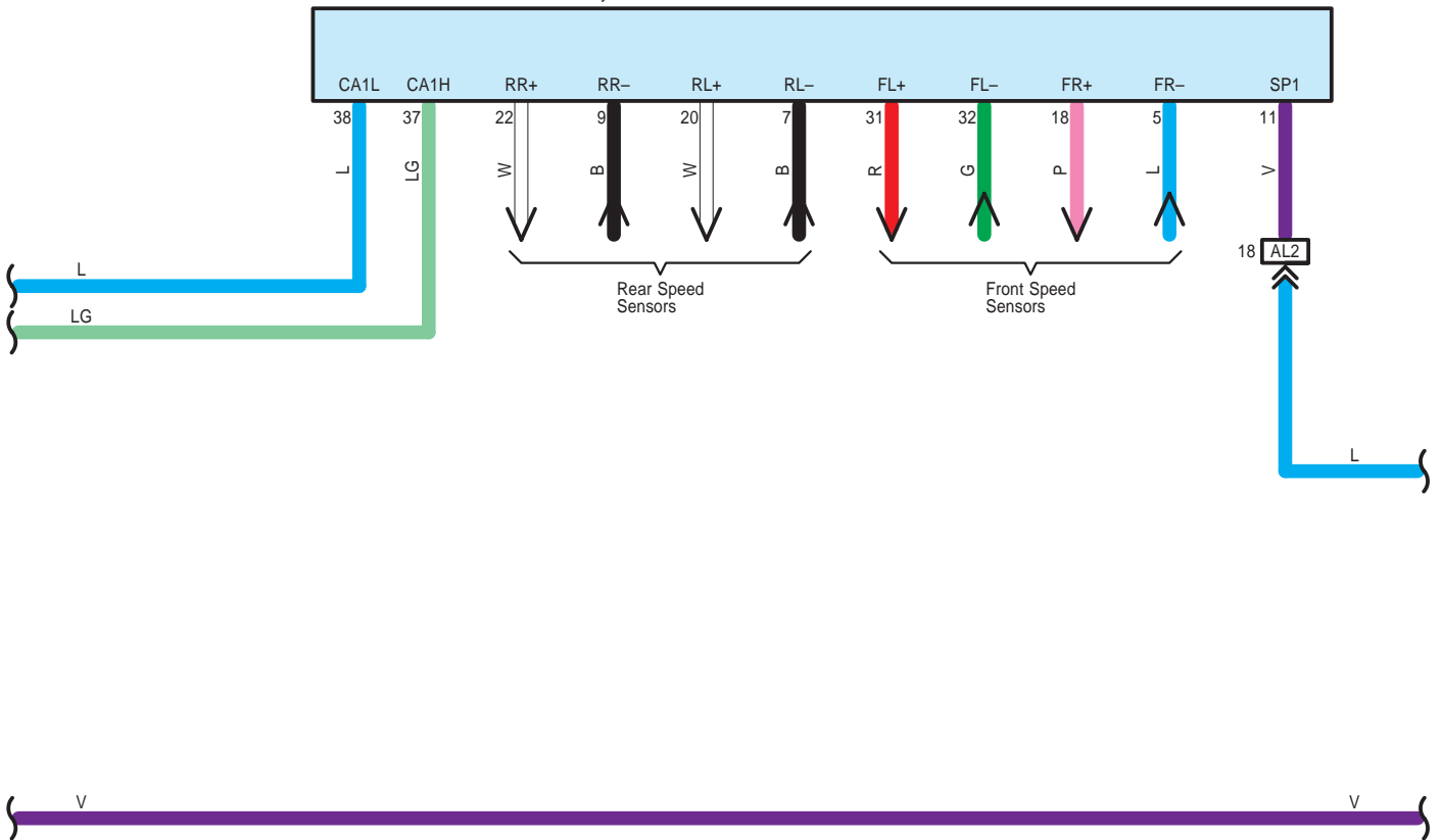
A58 Skid Control ECU with Actuator Assembly
