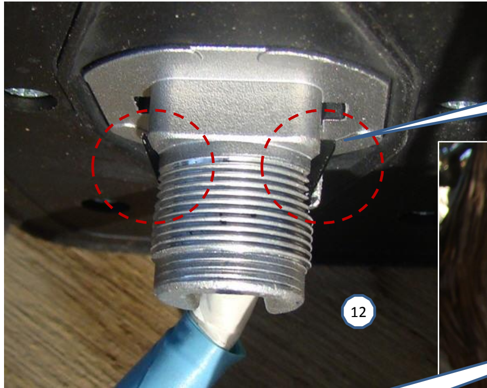
Press at Top of Threads after Nut Removed and Push Up Through Roof
