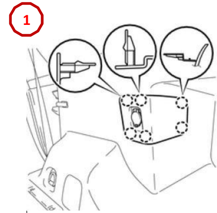
12v Power Outlet Panel Removed and Disconnected
