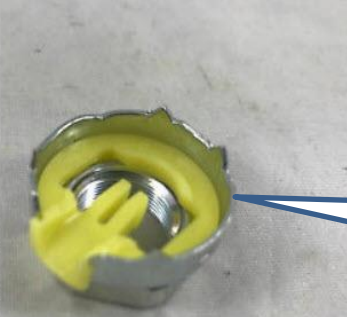
The Cable Exits through the Yellow Plastic Channel – Only the Nut Rotates
